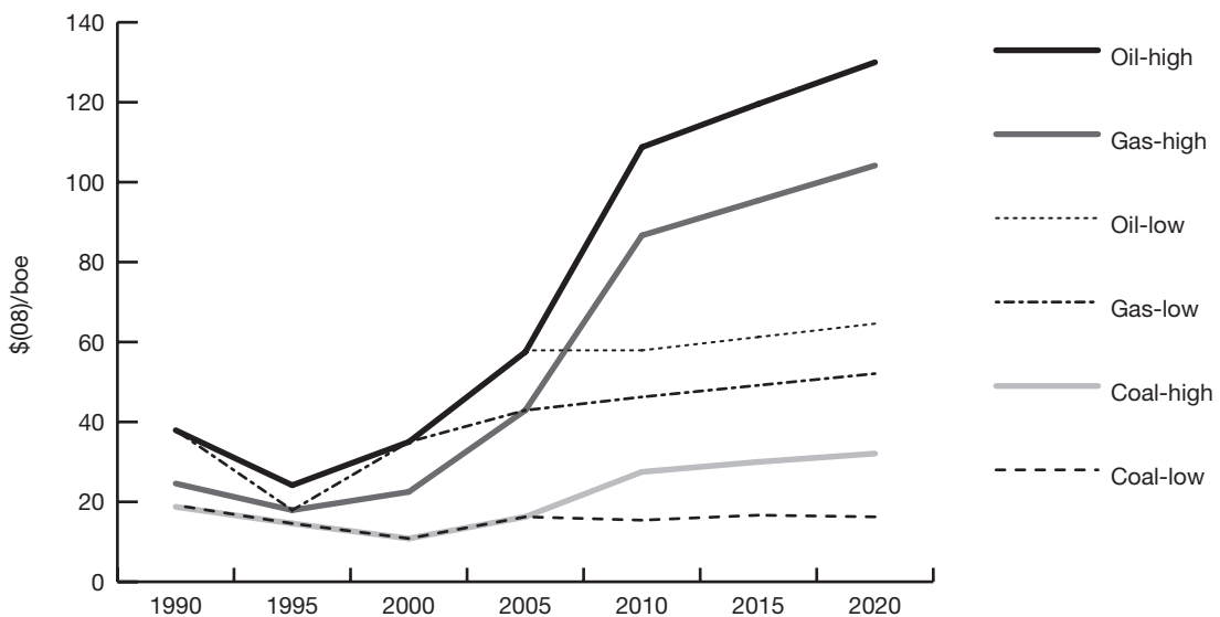
Figure 2.1 EU energy import prices in $ (2008)/barrel oil equivalent (boe)
