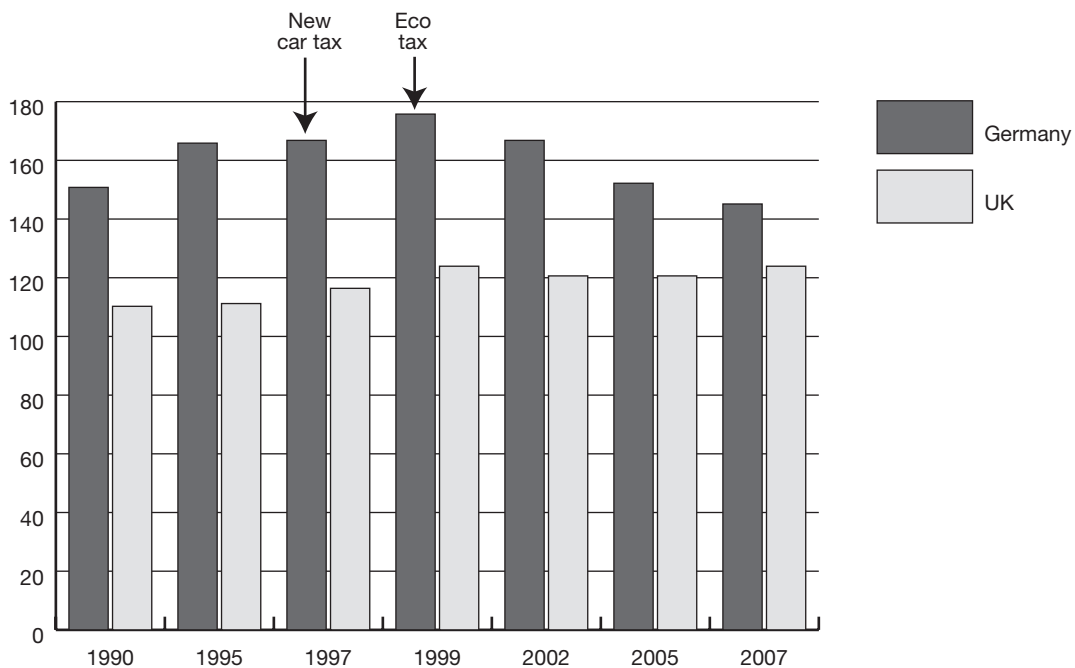
Figure 1.6 CO 2 emissions (Mt) of road traffic in Germany and UK 1990–2007
